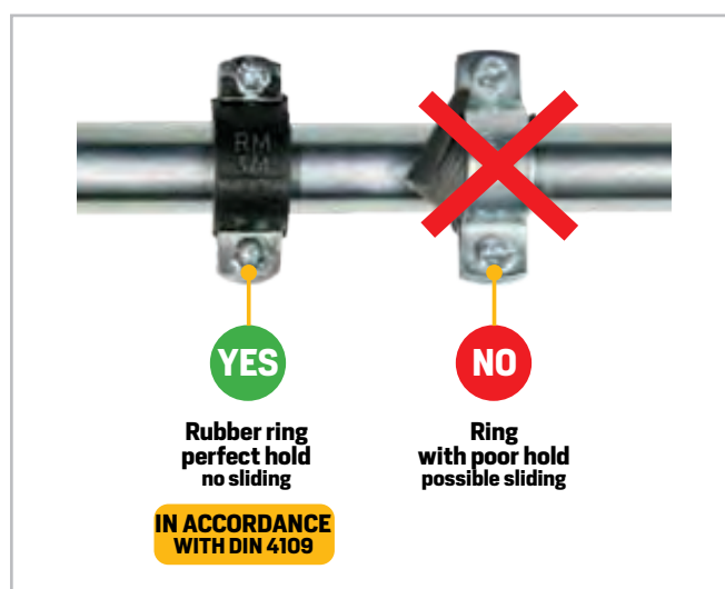
Figure 54 - Rubber ring PRATIKO in conformity with DIN 4109 (Unit RM Series 355/G - 351/G - 555/G - 156/G)
