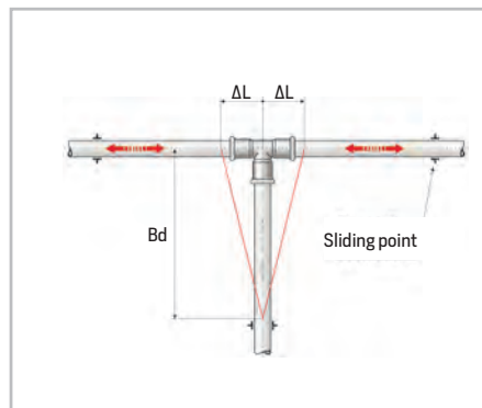
Figure 52 – Expansion compensation branch
