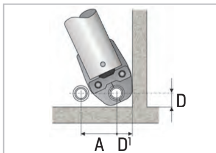
Figure 46 - Minimum distances and space requirements
