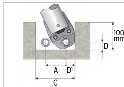
Figure 47 - Minimum distances and space requirements
