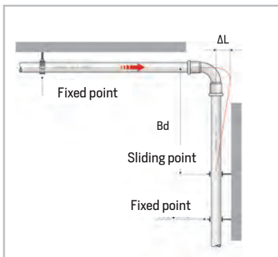
Figure 51 – Orthogonal-shaped expansion reach
