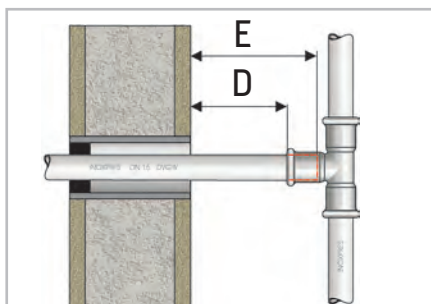
Figure 48 - Minimum distances and space requirements
