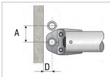
Figure 45 - Minimum distances and space requirements
