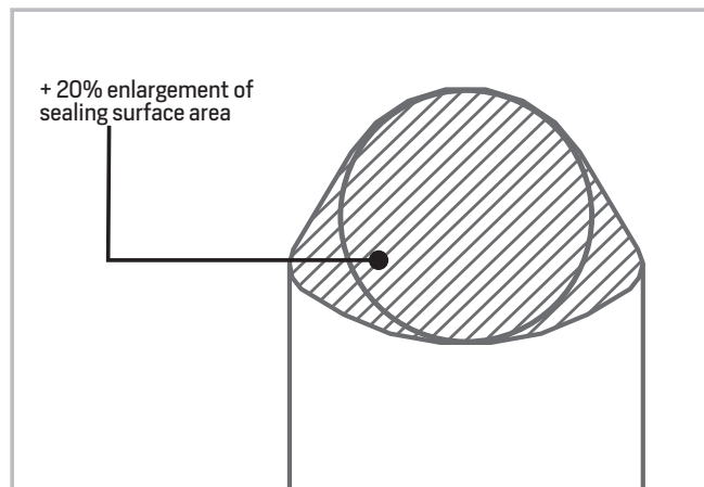
Figure 13 – Sealing ring profile
