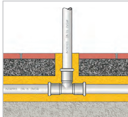
Figure 50b – Creation of expansion spaces
