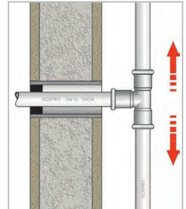
Figure 50c – Creation of expansion spaces
