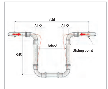
Figure 53 – U-bend Bd\Omega = Bd / 1,8
