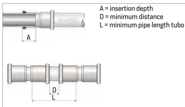
Figure 34 - Insertion depth and minimum dimensions
