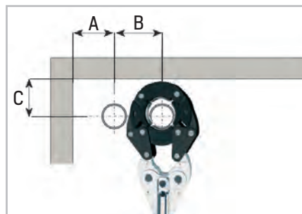
Figure 49 - Minimum distances for chains / collars
