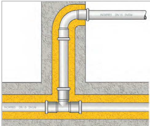
Figure 50a – Creation of expansion spaces
